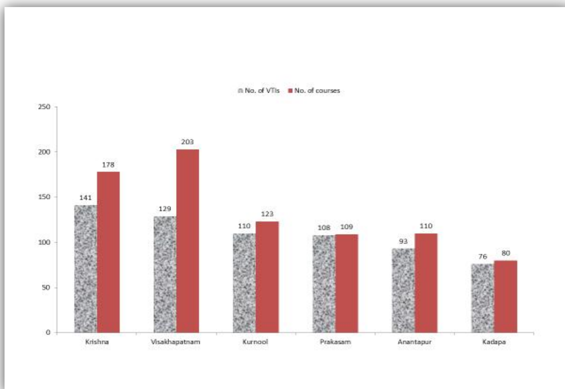
Figure 4.1 No. of VTIs in five Districts of AP
