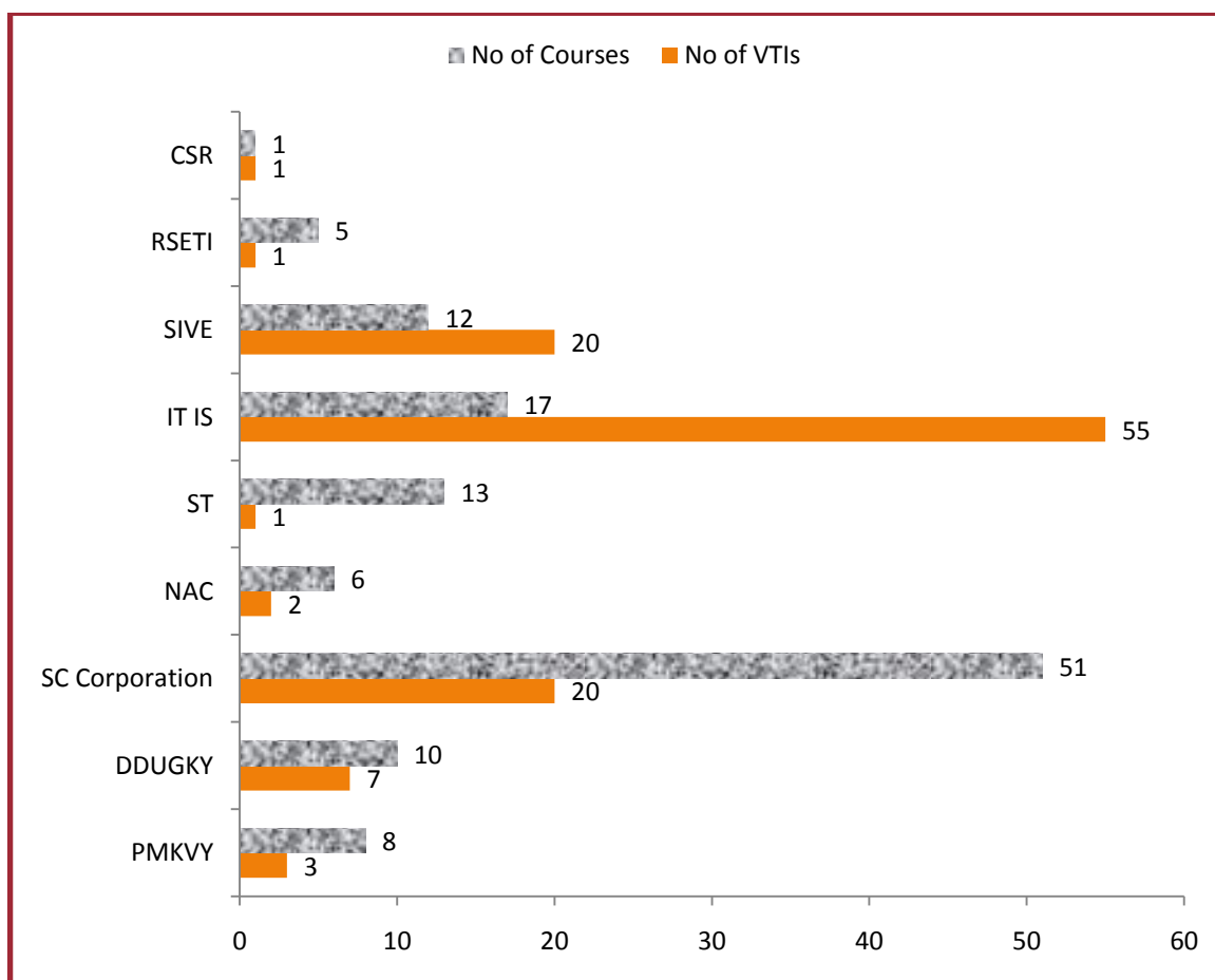
Figure 4.4 No. of VTIs in Kurnool District
