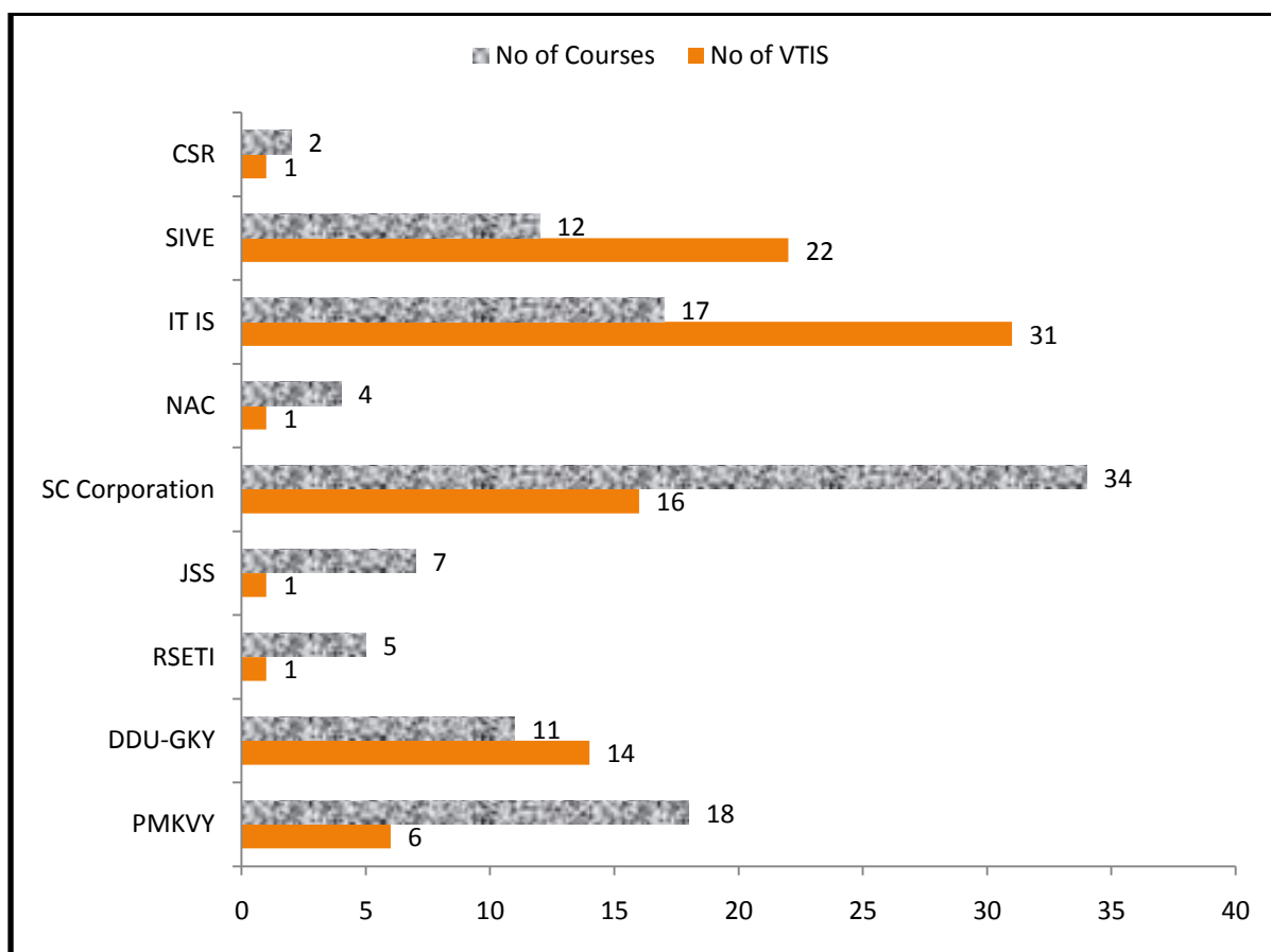
Figure 4.2: No. of VTIs in Anantapuram district
