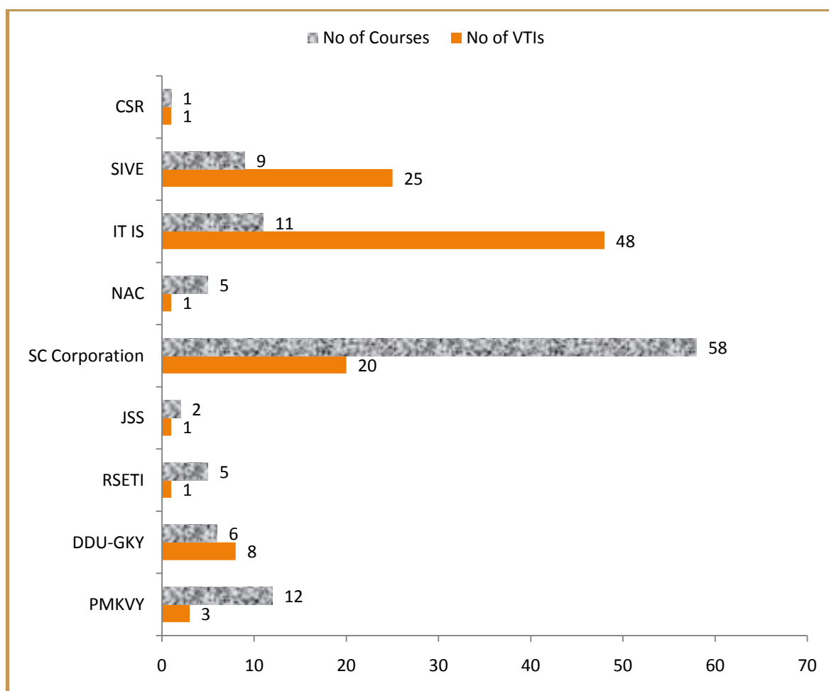
Figure 4.5 No. of VTIs in Prakasam District
