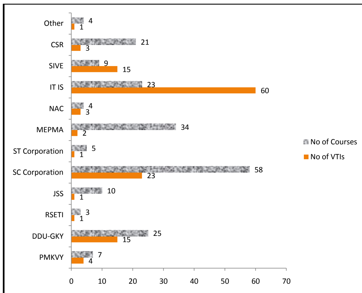
Figure 4.6 No. of VTIs in Visakhapatnam District
