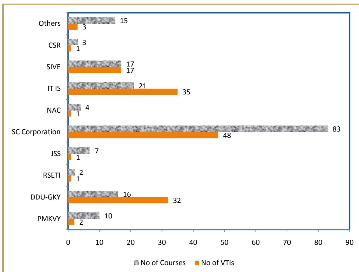
Figure 4.3 No. of VTIs in Krishna District
