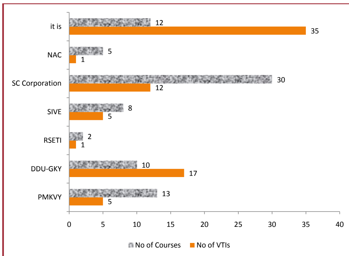
Figure 4.3: No. of VTIs in YSR Kadapa district
